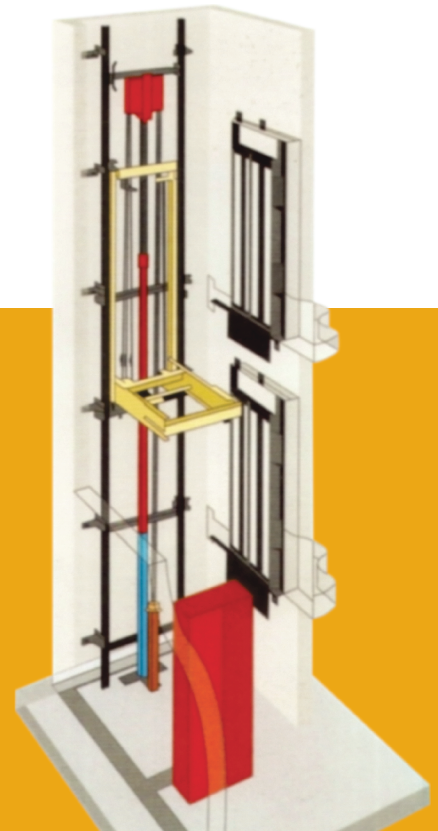
Single Cylinder Rope Type
